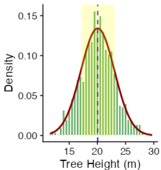
Can Fit Normal Distribution
