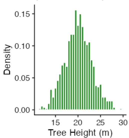
Normal Distribution (Tree Heights)
