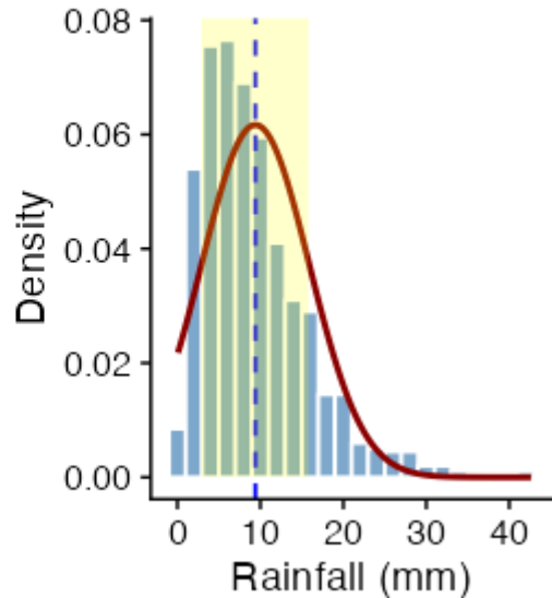
Can Fit Normal Distribution
