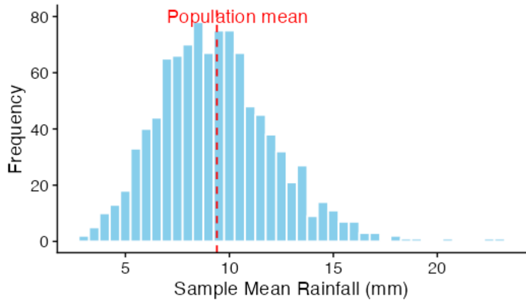
Distribution of Sample Means (n = 5)
