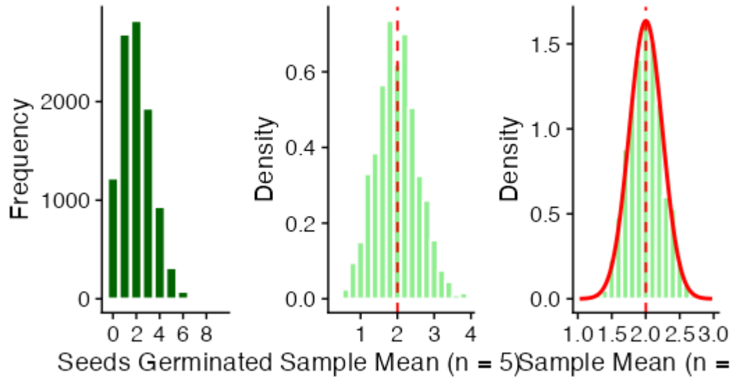
Original Population (Discrete & Skewed) Sampling Distribution of Small Samples Sampling Distribution of Larger Samples
