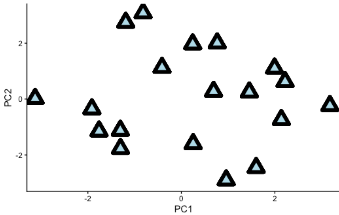
Our dataset with principle components 'PC1' and 'PC2' as the two viewing axes. Notice how the data is nicely spread out.
